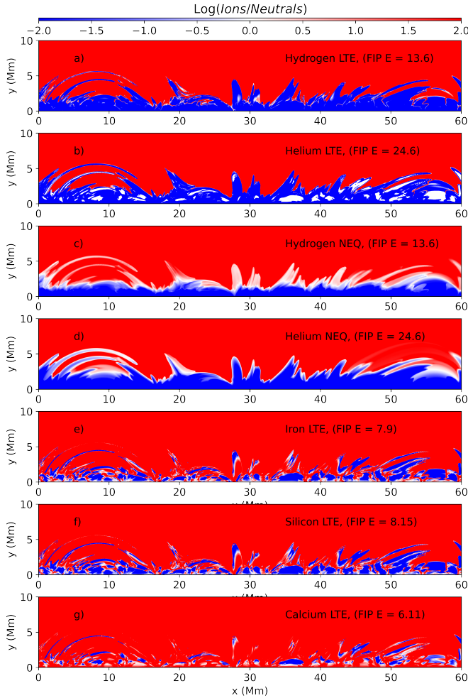
Figure 2. Ionization fractions are shown for various species with low and high FIP (hydrogen in panels a and c, helium in panels b and d, iron in panel e, silicon in panel f, and calcium in panel g). Panels a and b assume LTE, and panels c and d are in NEQ for hydrogen and helium. Note the color bar is in log-scale. Labels in the panels show the FIP energy in eV.
