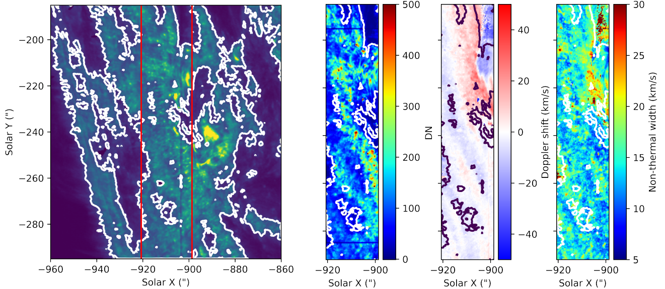
Figure 1. From left to right, IRIS SJI 1330 at 23:28:32, the total intensity, Doppler shift, and non-thermal width from Si IV 1339 Å from fitting a single Gaussian. The contours correspond to the SJI 1330 at 100 DN. The vertical red lines in the left panel limit the region of the raster scan.
