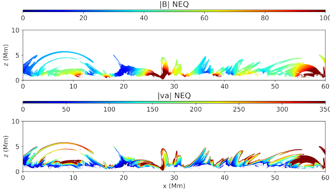
Figure 8. Magnetic field strength (top) and Alfvén speed (bottom) maps, where we applied the same mask as in panel h in Figure 5, reveal the complexity of the expansion or canopies of the magnetic field topology within the regions of interest.
