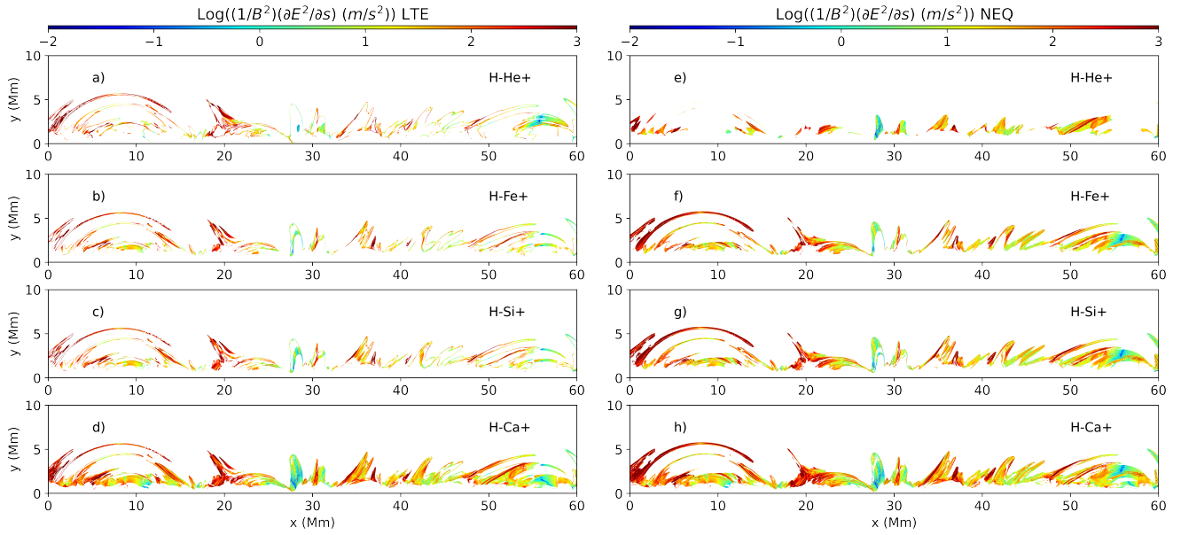
Figure 5. Maps of the electric field variations along the loop (Eq. 9). In these maps, we have masked out regions with high collision rates ( > 10 Hz) for each element (Figure 4) as well as regions where they have the same ionization state as hydrogen (Figure 3). The region of interest (non-masked region) is where the ponderomotive force may produce chemical fractionation. The distribution of the various panels is the same as in Figure 4.
