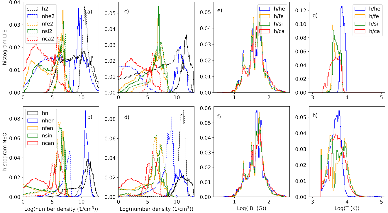
Figure 7. Histogram of the density population for neutrals (solid, panels a-d) and ions (dashed, panels a-d), magnetic field (third column) and temperature (right column) within the regions of interest (non-masked out regions) in Figure 5, for each species (panels a and b, and e-h). Panels c and d are for the region of interest of H-Ca. LTE case is in the top row and NEQ in the bottom row.
