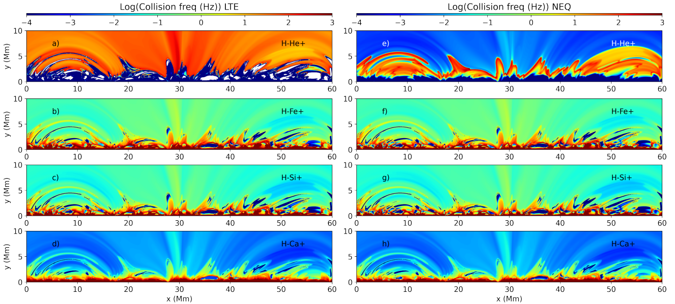
Figure 4. Collision frequency between the neutral hydrogen and the other ionized species (helium, iron, silicon, and calcium from top to bottom) maps are shown in LTE (left column) and NEQ ionization (right column).
