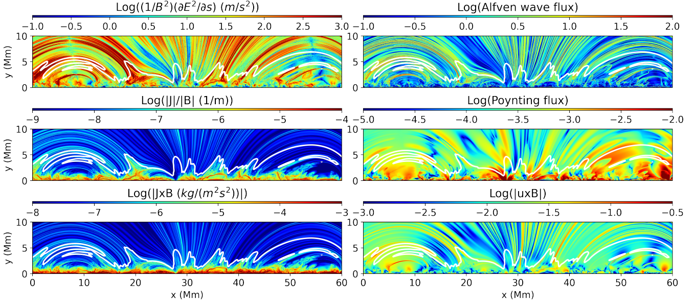
Figure 6. Various physical processes play a different role in different features. \delta_s E following Eq 9, the Alfvén wave power, |J|/|B| , Poynting flux, Lorentz force and advection term of the electric field are shown from left to right and top to bottom, respectively. The solid line is at temperature 10^5 K.
