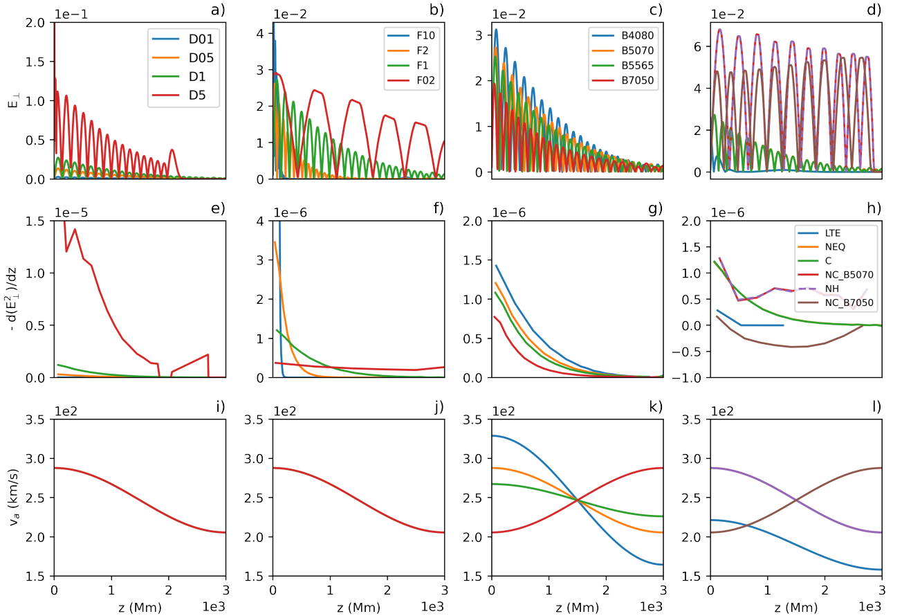
Figure 14. Electric field perpendicular to the magnetic field (top row), -dE_{\perp}^2/dz (middle row) and Alfvén speed (bottom row) as a function of z -axis. We show this for a variety of simulations with varying amplitude, and varying frequency of the Alfvén wave driver, the variation of the guide magnetic field, and different physical assumptions, as shown, respectively, from left to right.
